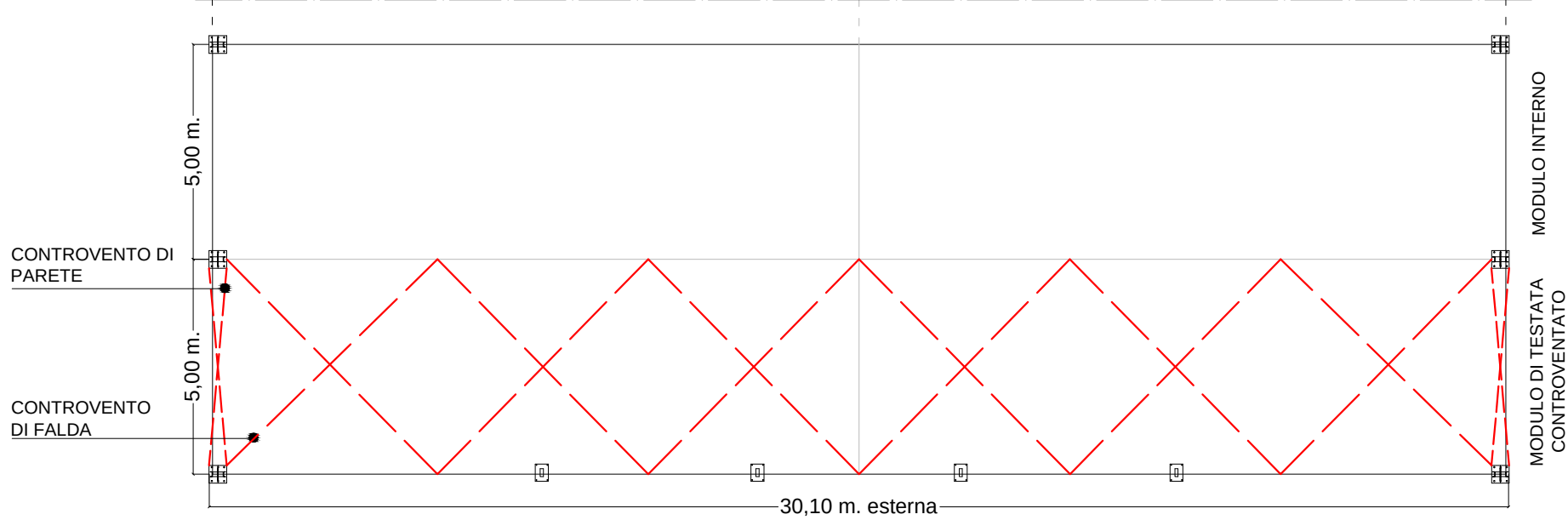
PLANIMETRIA MODULI STANDARD
