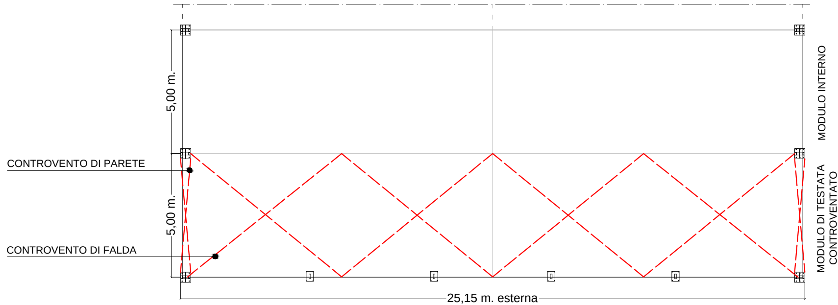
PLANIMETRIA MODULI STANDARD
