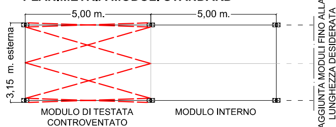
PLANIMETRIA MODULI STANDARD
