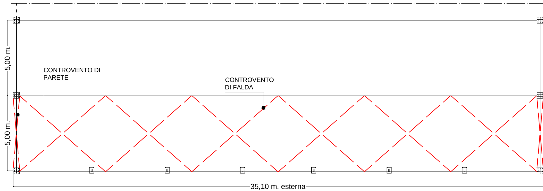
PLANIMETRIA MODULI STANDARD
