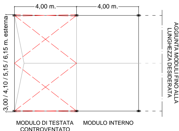
PLANIMETRIA MODULI STANDARD
