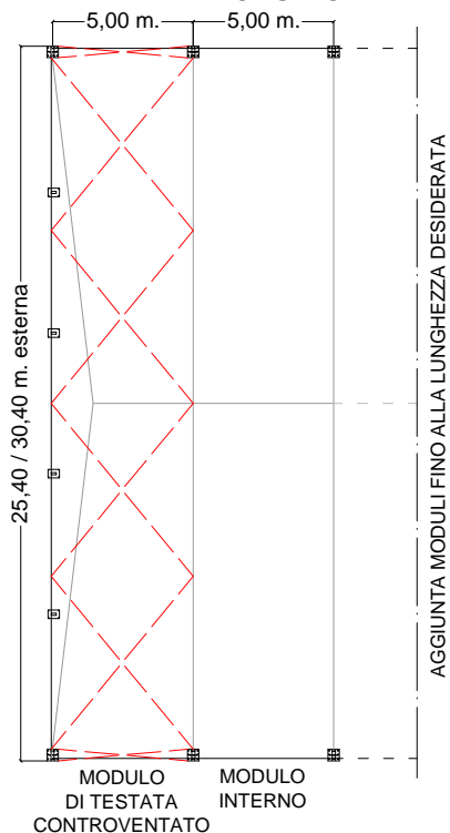
PLANIMETRIA MODULI STANDARD
