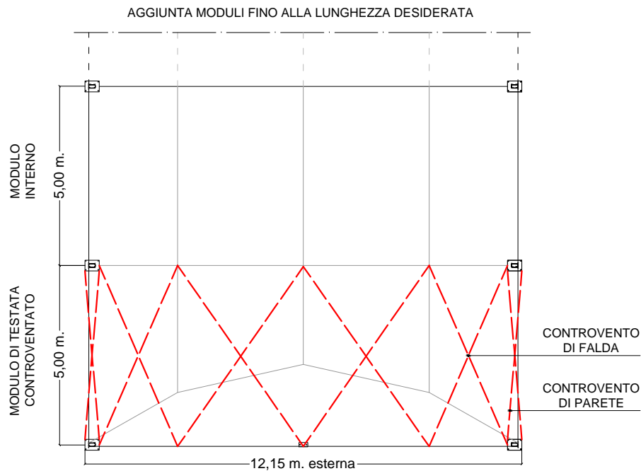
PLANIMETRIA MODULI STANDARD
