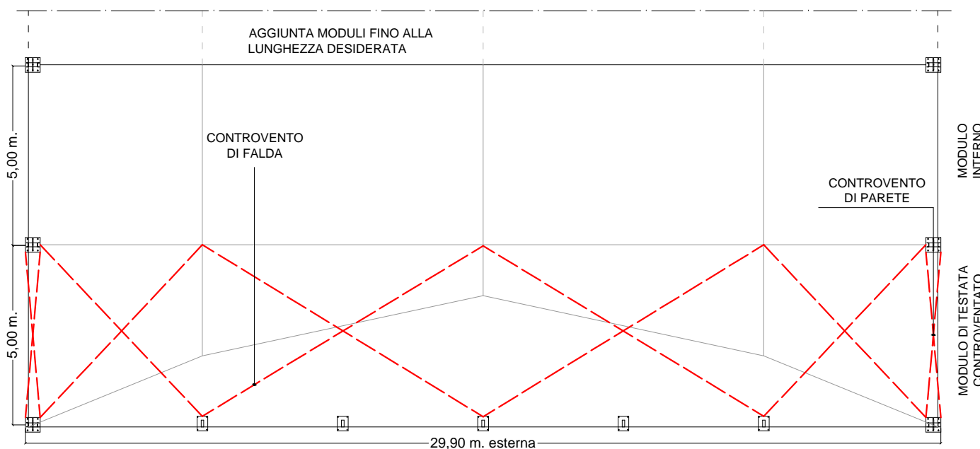
PLANIMETRIA MODULI STANDARD
